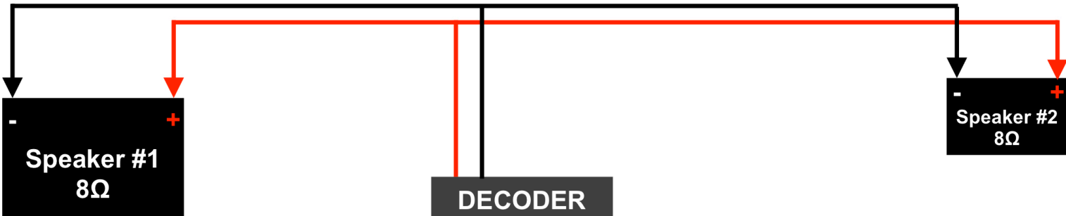
Parallel Wiring of two 8Ω Speakers for 4Ω Total Load
