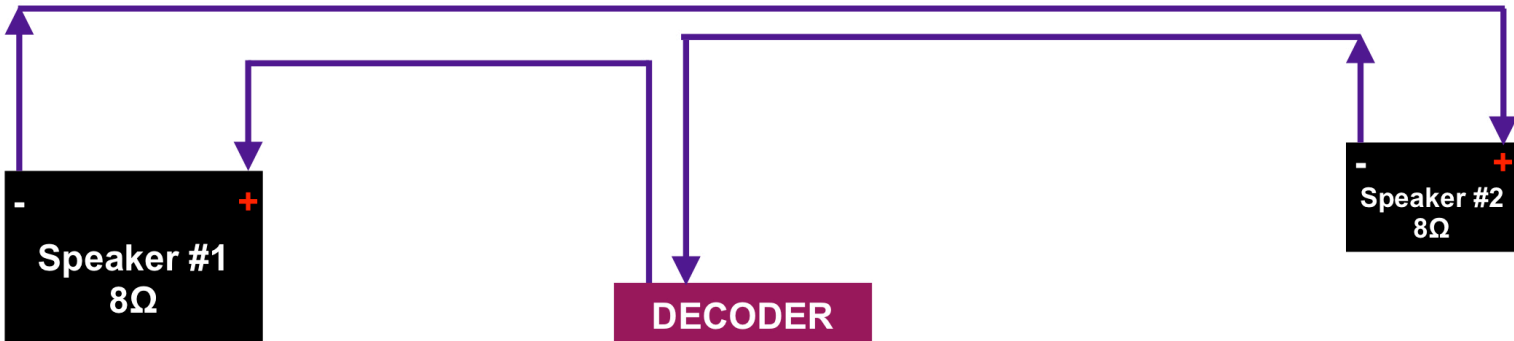
Series Wiring of two 8Ω Speakers for 16Ω Total Load
