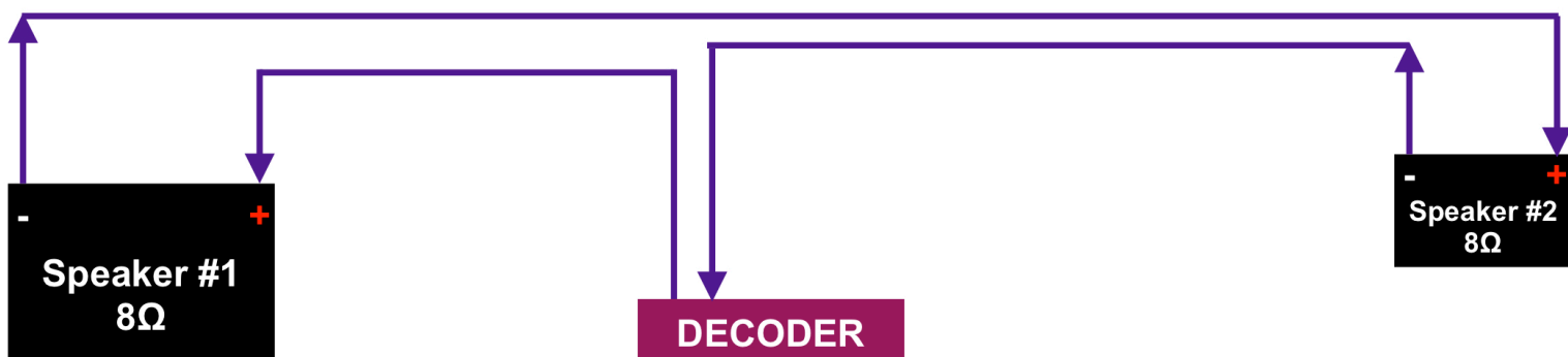
Series Wiring of two 8\Omega Speakers for 16\Omega Total Load
